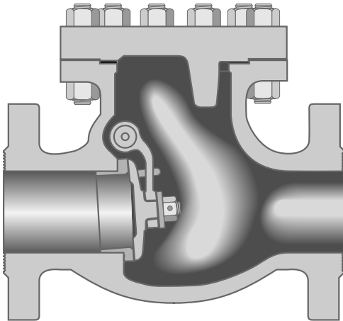
Figure 60-SF-U Flanged
