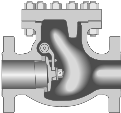
Figure 30-SF-U Flanged
